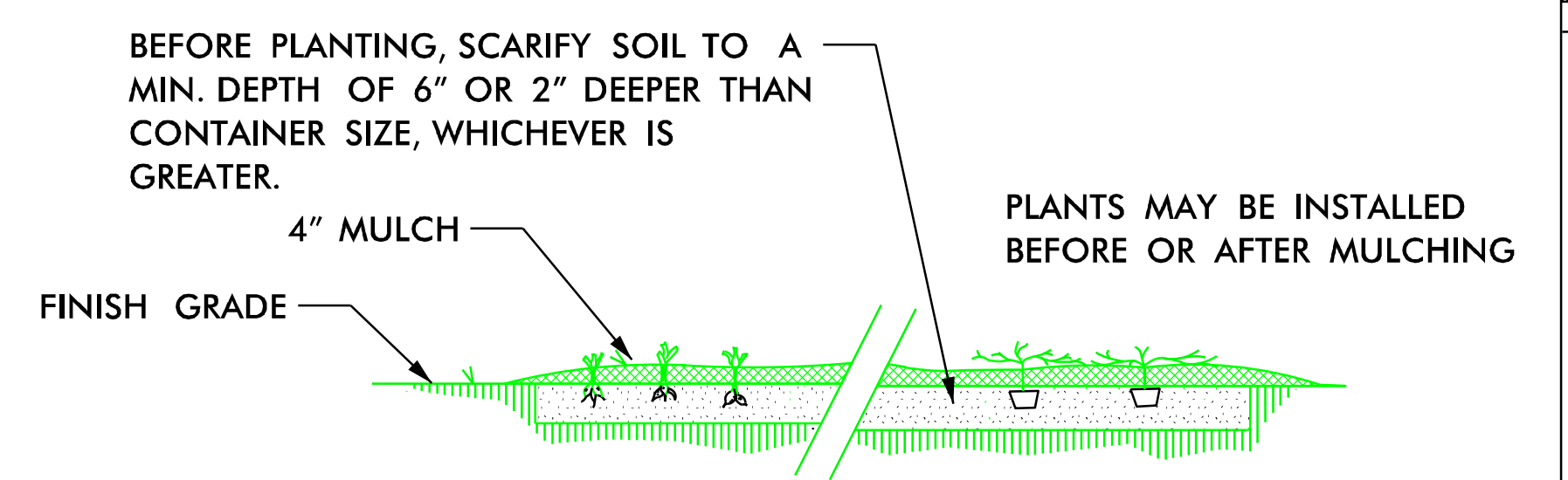
GROUND COVER/BEDDING PLANT DETAIL
