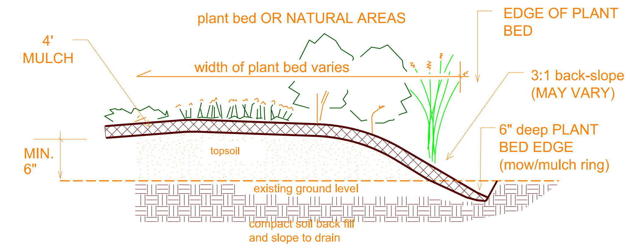
PLANT BED EDGE DETAIL
